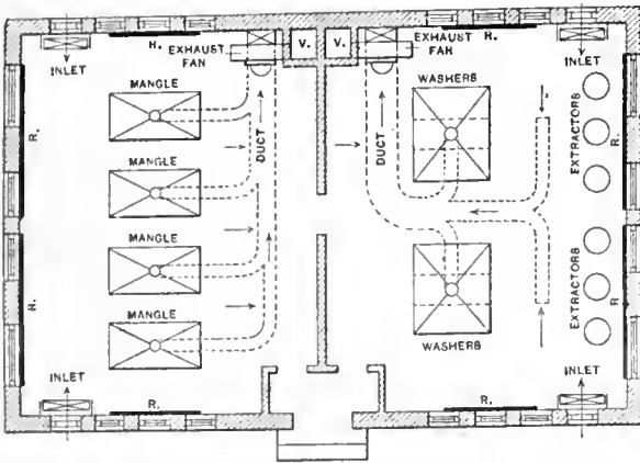
FIG. 8. TYPICAL ARRANGEMENT FOR A LAUNDRY
